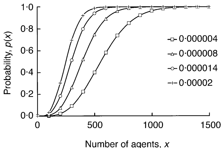
Fig. 2. Probability of establishment curves p(x) for inocula of different sizes, x . The curves are defined by p(x) = p_m(1 - e^{-ax})^2 , and the value of a alters the steepness of the curve.
