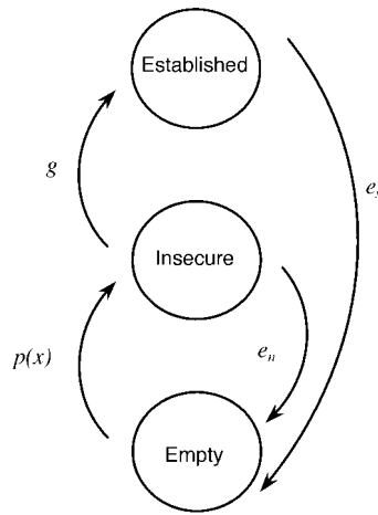
Fig. 1. State transitions in the metapopulation model for an individual site. The system can be in one of three possible states: empty, insecure or established. Transitions between these states can occur due to the processes of colonization ( p(x) ), extinction ( e_s and e_n ) and growth ( g ).
