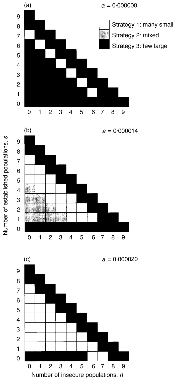
Fig. 3. Optimal strategy sets for a increasing from (a) a = 0.000008 to (b) a = 0.000014 to (c) a = 0.000020 . All other parameters are as defined for the baseline scenario (Table 1). Each box represents a possible state of the system, and the key indicates the optimal decision to make for that particular state. Note that when there are no empty sites available, no releases can be made.
